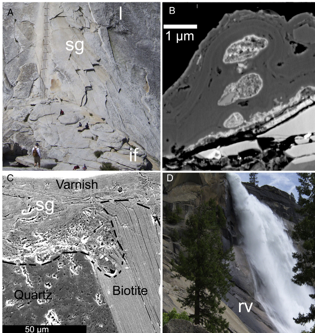
Fig. 7. Connecting field setting to electron microscopy of rock coatings on Half Dome, Yosemite National Park, California. (A) Many different types of rock coatings can be found at the base of the Half Dome ladder, including iron films (if), silica glaze (sg), and lithobionts (l). (B) Bacterial-sized cocci form encapsulated by the silica glaze seen in image A. The outermost portion of the cocci form is bright because it contains the most manganese and iron enrichment. (C) Rock varnish found in a dark streak on Half Dome (image D). Note how the rock varnish forms a distinct contact on both quartz and biotite. However, other types of rock coatings can interrupt varnish accretion, such as the small pocket of silica glaze (sg). (D) The dark stains in Yosemite Valley are composed of many different types of rock coatings, including rock varnish (rv).
