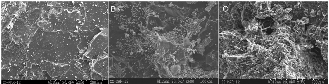
Fig. 14. Scanning electron micrographs of sandstone samples from the Ouachita Mountains, Arkansas, showing (A) the surface of a fresh sandstone clast removed from an upturned root wad (<10 years old); (B) the surface of a root groove on a large sandstone boulder, which has an abundance of organic material, iron-rich florets, and pitted sand grains; (C) 1.5 mm below the root groove surface, where the rock has been bleached, and the sand grains are heavily pitted in association with the endolithic microbes and roots.
