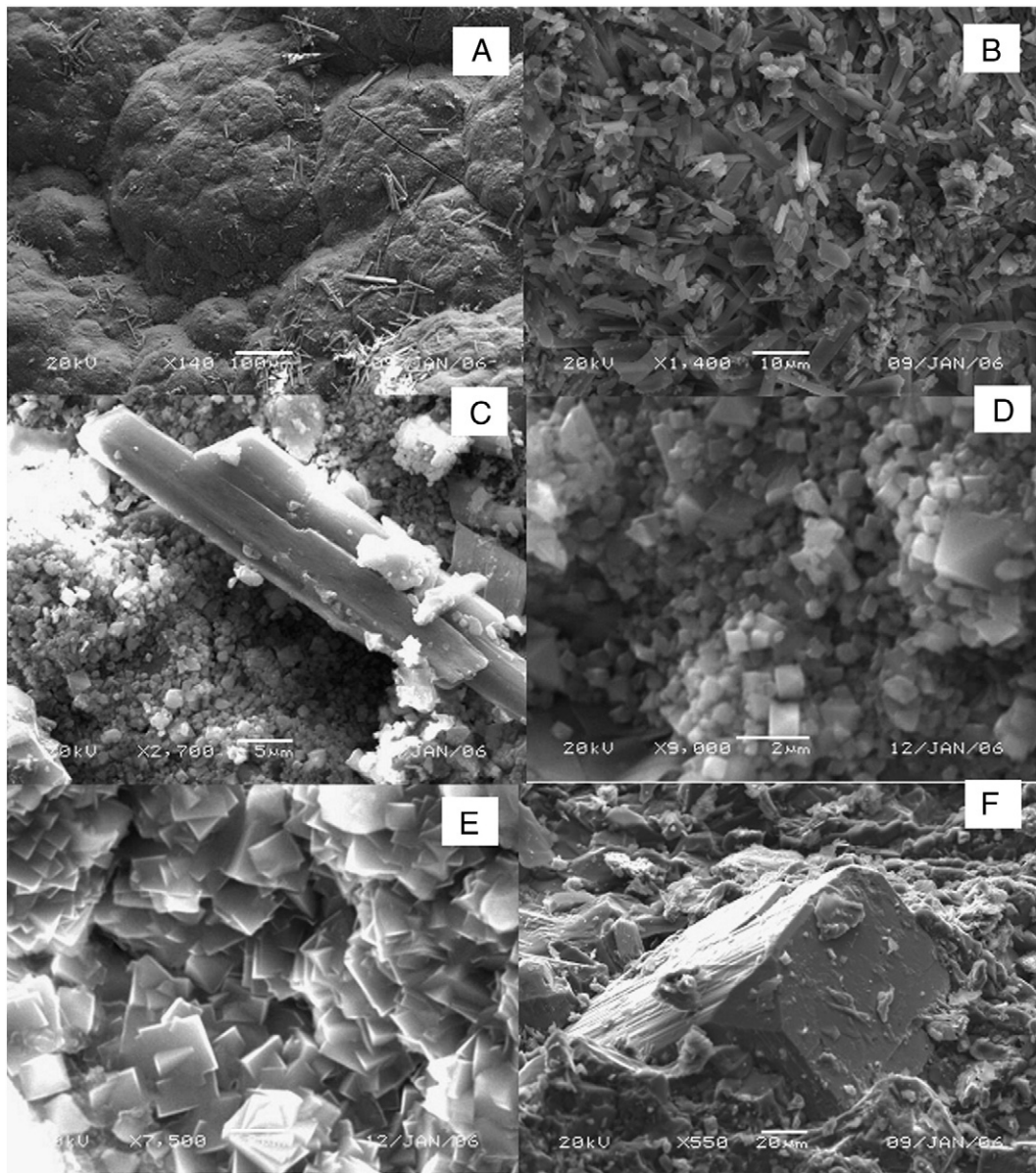
Fig. 3. Field investigations identified protected boulder sites where a variety of rock coatings occurred. Subsequent electron microscopy and X-ray diffraction analysis showed these coatings to contain gypsum (A and B), often associated with jarosite (C–E), and all of the coatings to be associated with pyrite and its oxidation (F).
