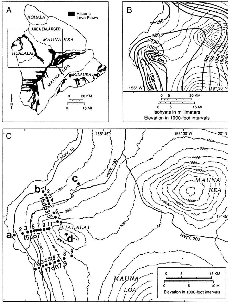
Fig. 10. The dated lava flows of Hualalai volcano (A) Hawaii (Moore and Clague, 1991) provide varied field sites where rainshadow effects allow isohyets to cross different elevations (B) allowing the sampling of lava flow surfaces (C) along different isotherms, different isohyets, under lichens, and also avoiding lichens and fungi.
