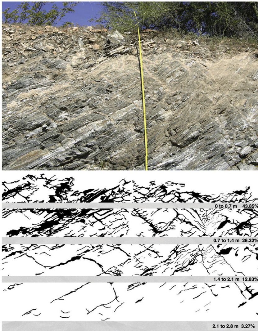
Fig. 11. Road excavation cut into the Gila Range, central Arizona, where digital image processing generated a map of the carbonate veins in bedrock. The decrease in abundance is typical of this carbon pool.
