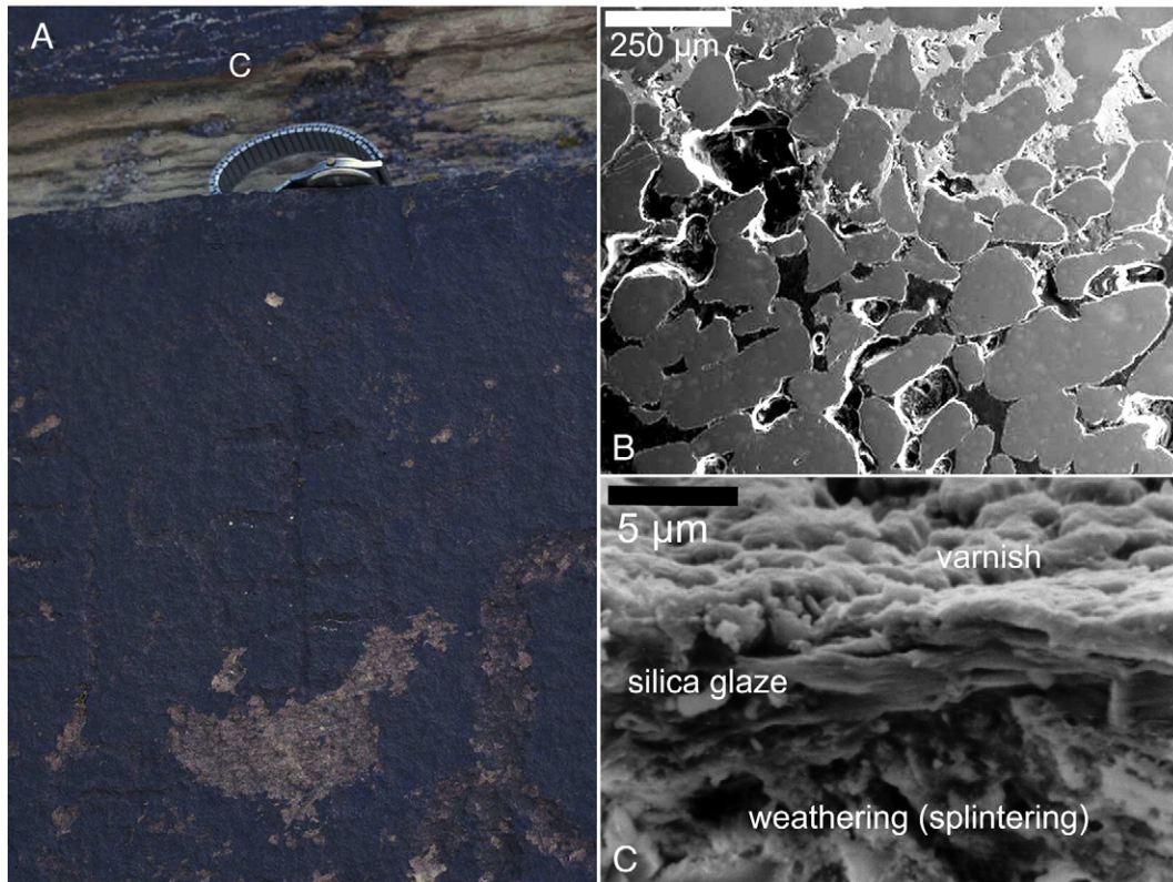
Fig. 8. Case hardening of sandstone at Petrified Forest National Park. (A) A case hardened joint face forms a stable surface used for carving of a bird motif and an earlier anthropomorphic image. Note, however, that the case hardening has been breached—with wristwatch for scale. (B) Back-scattered electron microscope image of a cross section collected at location “c” in image (A). The bright material between the grains is a heavy metal skin of iron and manganese constituents, likely dissolved from rock varnish and mobilized into the sandstone to stabilize the upper millimeter of a surface. Note, also, the abundant porosity underneath the case hardened heavy metal skin. Once the case hardening is breached, this porosity makes erosion rapid. (C) Another type of case hardening exists at the very surface of this panel. A mixture of silica glaze and rock varnish can offer additional stability in the upper few microns, where this secondary electron image was from a sample also collected from the letter C above the watch in image A.
