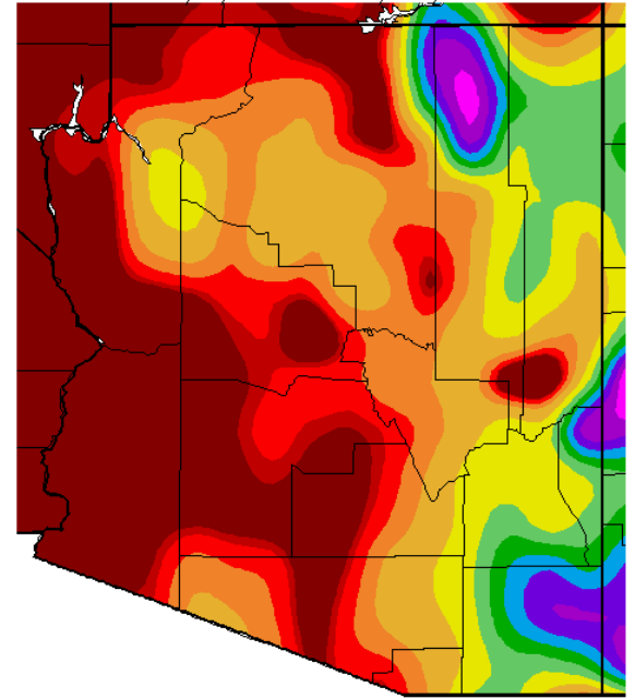
Total Precipitation (in.) 3/1/2009 – 3/31/2009
