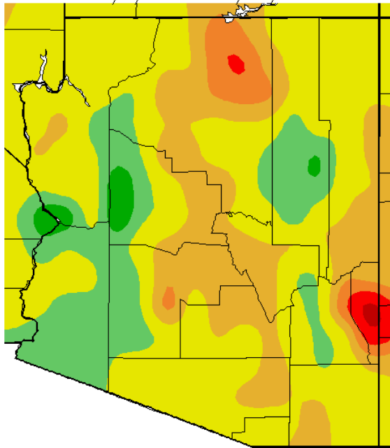
Av. Min. Temperature dep from Ave (deg. F) 1/1/2009 - 3/31/2009
