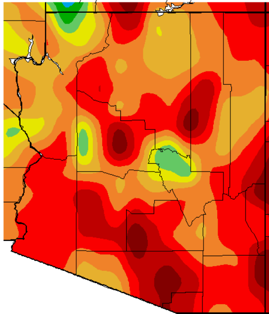
Av. Max. Temperature dep from Ave (deg F) 3/1/2009 - 3/31/2009
