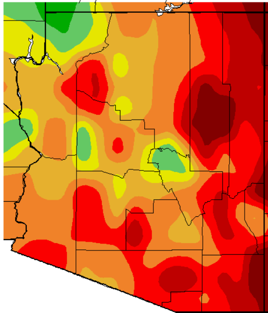
Av. Max. Temperature dep from Ave (deg F) 1/1/2009 - 3/31/2009
