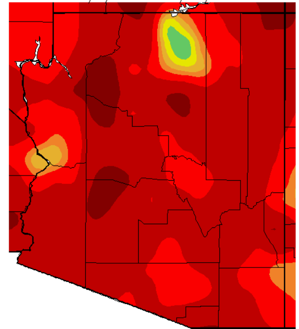
Percent of Average Precipitation (%) 1/1/2009 - 3/31/2009
