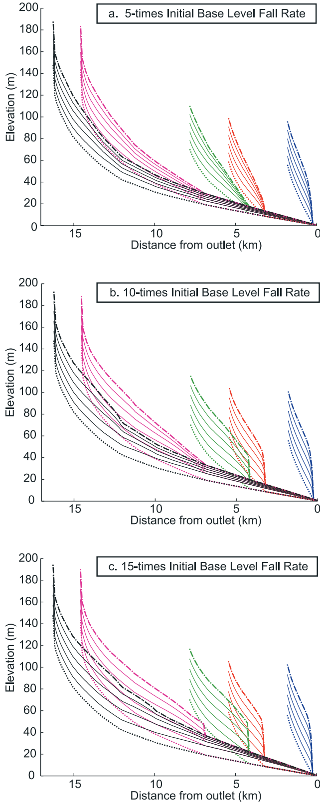
Figure 7. Formation of permanent hanging tributaries in the saltation-abrasion model requires sufficiently fast main stem incision rates. This figure examines tributary response given three different rates of progressive base level fall. (a) For 5\times the initial base level fall rate, only the two tributaries with the smallest drainage areas (the two closest to the outlet) form a hanging valley. (b) For 10\times the initial base level fall rate, all three of the smallest tributaries near the outlet form hanging valleys. (c) For 15\times the initial base level fall rate, all tributaries in the basin become hanging valleys. For each hanging tributary, the incision rate in the main stem outpaces the incision rate at the tributary junction. If the progressive base level fall is sustained, the hanging tributaries will increase in elevation indefinitely. Depending on the slopes of the oversteepened reaches ( S_{junction} ), once the base level fall rate returns to the background rate, the tributaries either will remain as permanent hanging valleys (if S_{junction} > S_{hang} ) or will gradually reestablish grade with the main stem channel (if S_{junction} < S_{hang} ).
