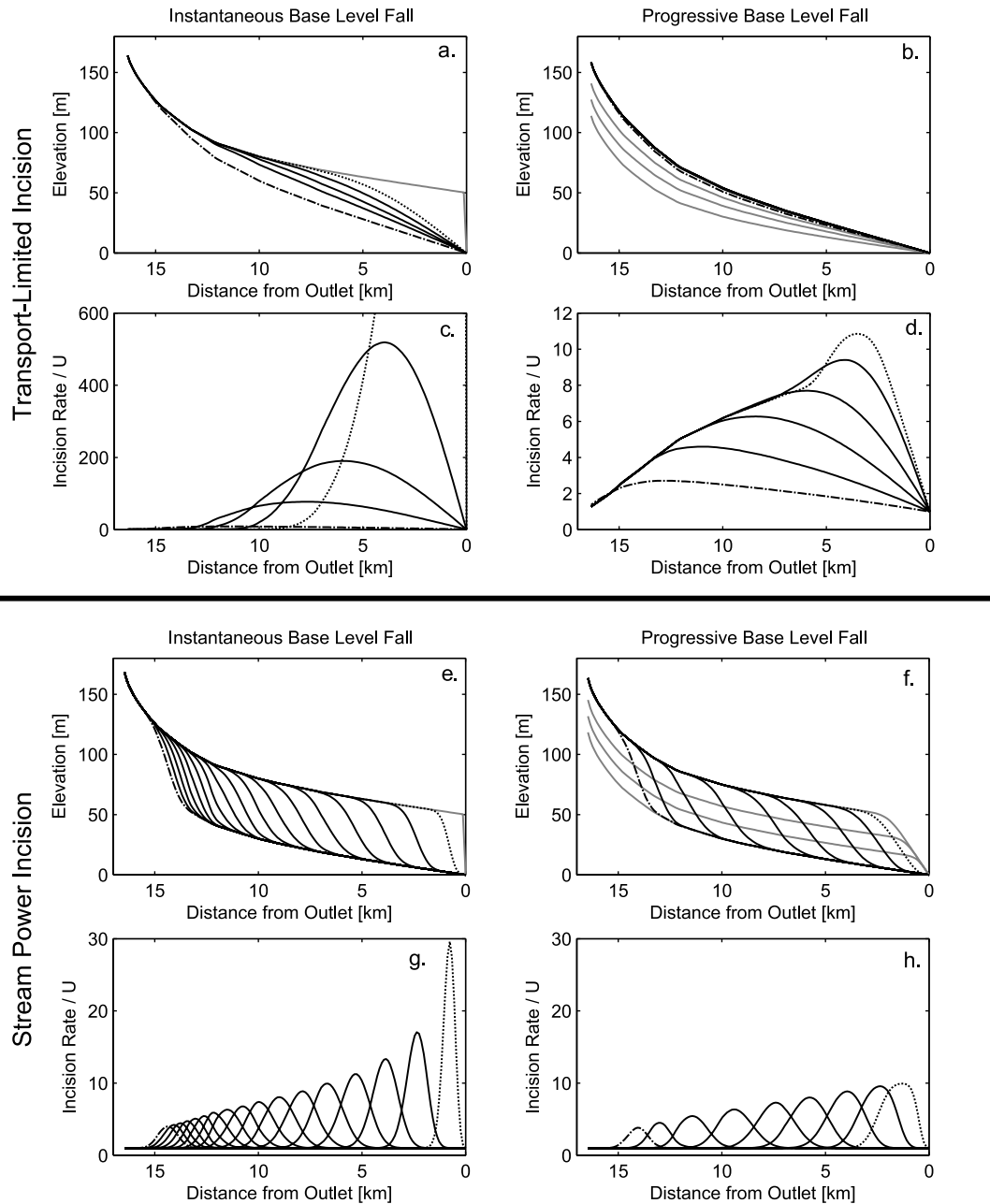
Figure 4. Numerical simulations of main stem profile evolution and normalized incision rates are observed following base level fall. Normalized incision is calculated by dividing the incision rate by the long-term, predisturbance background rate of base level fall. Shown are (a–d) plots that reflect simulations governed by the transport-limited (T-L) incision rule and (e–h) plots that reflect simulations governed by the stream power (S-P) incision rule. In Figures 4a and 4e, the gray line represents the channel profile immediately after the base level fall; the dotted line represents the first profile illustrated after the base level fall; and the dash-dotted line is the final profile illustrated. In Figures 4c and 4g, the dotted and dash-dotted lines illustrate the incision rate for the dotted and dash-dotted profiles in Figures 4a and 4e, respectively. In Figures 4b and 4f, gray lines reveal the evolution of the channel profile during progressive base level fall (no incision rates are shown for these times), and the dotted lines represent the first profile shown after the base level fall rate returns to the background rate; the dash-dotted line is the final profile shown. In Figure 4b, the profile changes very slowly, and therefore the differences between each time plotted are not discernable (plotting times were chosen to show the pattern in incision rate). Note that the y axis differs between Figures 4c and 4d. In each of the plots, the time between each channel profile and incision plot is not necessarily steady; rather, the times plotted were chosen to illustrate the general behavior of the system. Note that the incision signal in the S-P case migrates up the main stem as a discrete step, while in the T-L case, the increase in high sediment delivery during the transient prevents the downstream reaches from reequilibrating.
