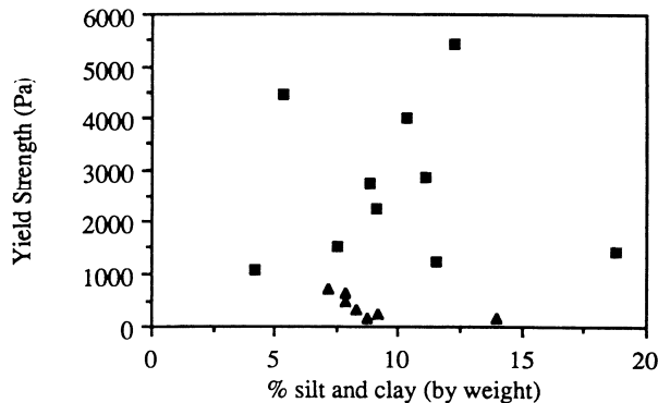
Figure 11. Estimated yield strength plotted against percentage of silt-and-clay in the matrix for all debris-flow deposits for which sieve analyses are available. No overall correlation is evident. Triangles represent debris-flow deposits at the distal margin of the bajada and suggest a second-order correlation with silt-clay content.
