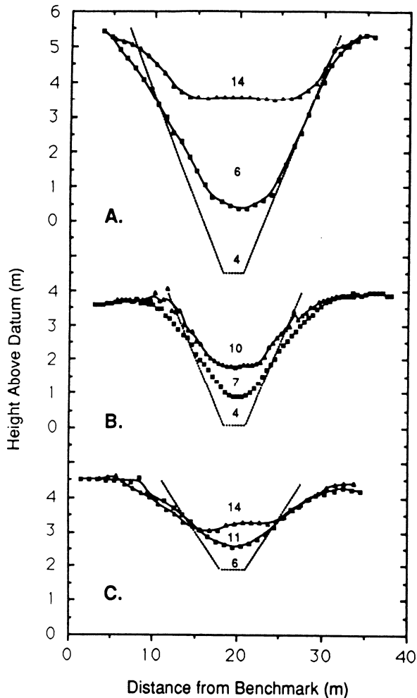
Figure 6. Surveys of representative channel cross sections, plotted at a 4× vertical exaggeration. For each channel, a survey immediately upstream of a debris-flow plug (triangles) is compared with a survey immediately downstream of that plug (squares). Width-to-depth ratios are indicated for each channel section. The steep-sided, flat-floored channel cross sections shown for comparison (dotted lines) are referred to in the discussion of channel formation (see also Fig. 9). (A) Deeply incised channel on upper Pinyon Creek fan. (B) Typical channel on upper Pinyon Creek fan. (C) Channel typical of the lower bajada (located 6 km from the range front).
