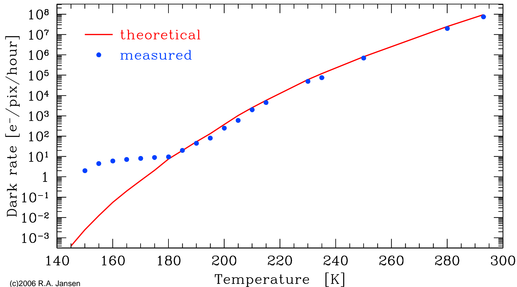
Figure 10: Measured and expected temperature dependence of the dark rate for a thinned back-illuminated 2k \times 4k EEV CCD delivered to ESO. Below \sim 180 K, the measured dark rate does not diminish as expected due to other residual effects. Nonetheless, this particular device reaches a dark current of only \sim 2 e^-/\text{pix}/\text{hour} when operated at 150 K.
