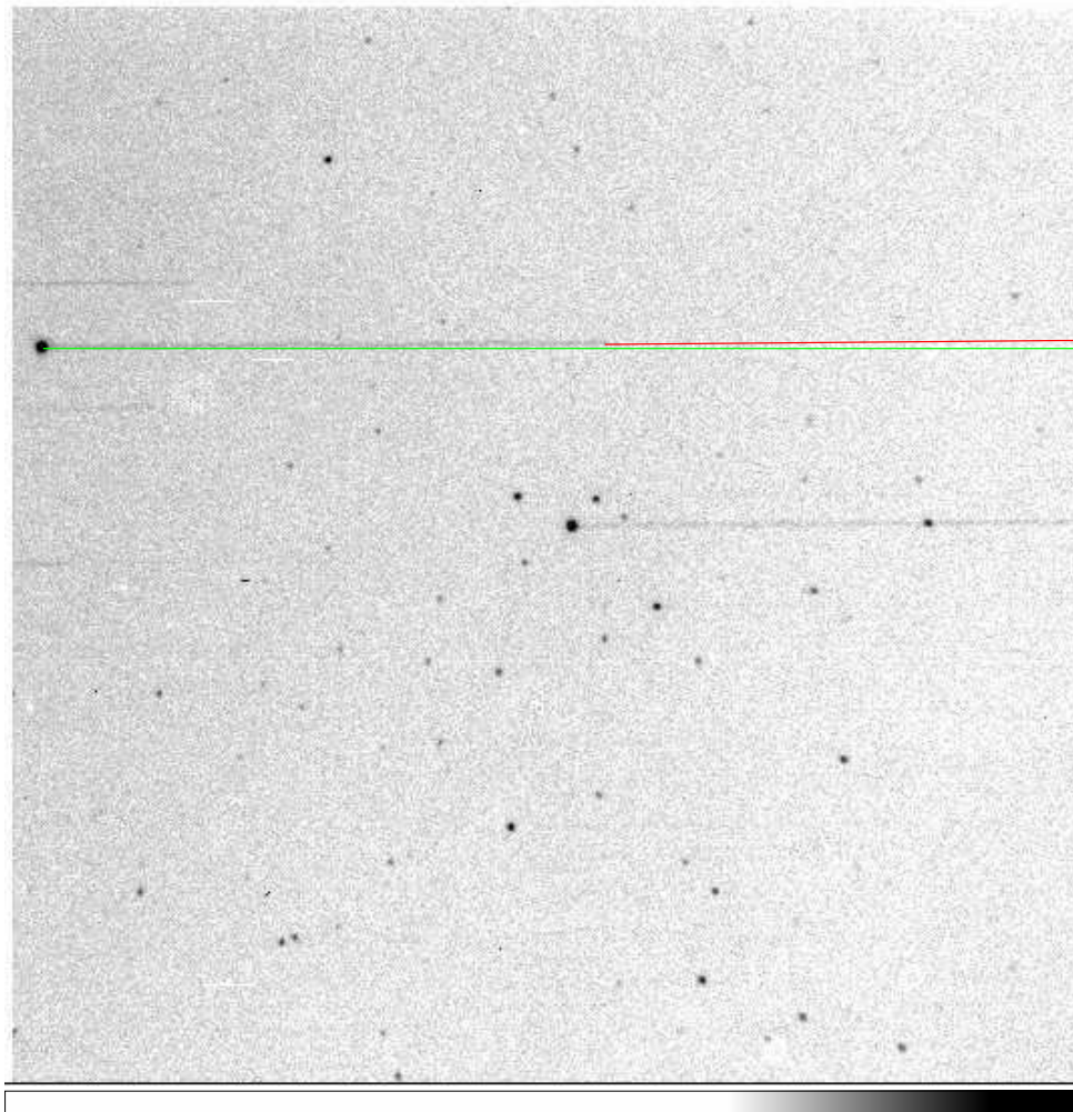
Figure 29: Example of a CCD orientation exposure, obtained at the FLWO 48" telescope. The star trail points W from the stellar image. In this case, the the CCD was rotated \sim 0^{\circ}.4 E of N.
