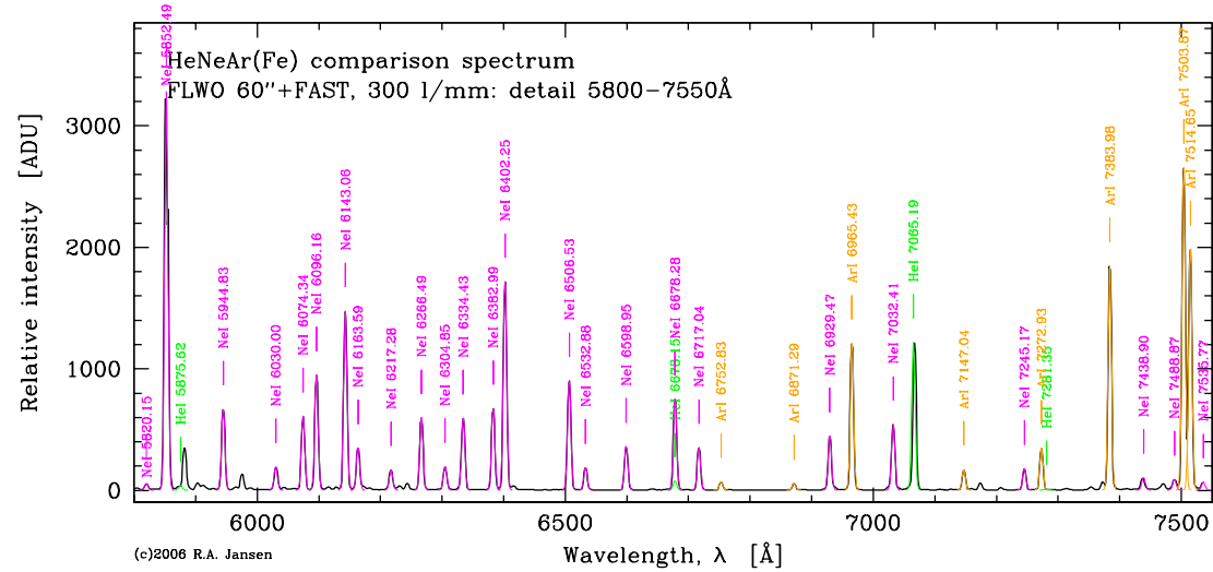
Figure 32: (cont'd) The region between 5000Å and 6500Å ( top ) and that between 5800Å and 7550Å ( bottom ).
