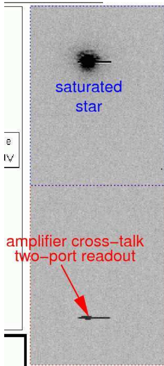
Figure 18: Example of crosstalk in an EEV 44-82 2k \times 4k CCD.
