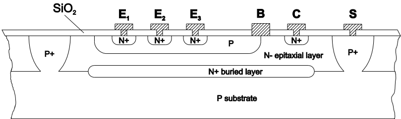
Multi-emitter Schottky BJT
