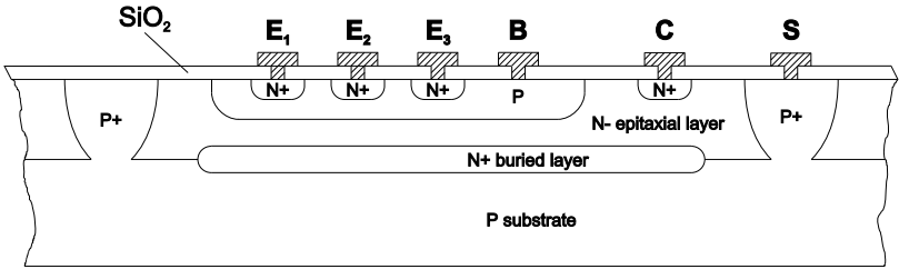
Multi-emitter BJT
