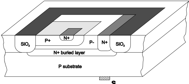
Oxide Isolated
