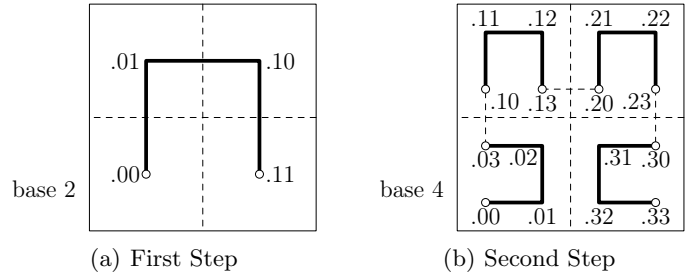
Fig. 1. The Generation of 2 Dimensional Hilbert Curve
