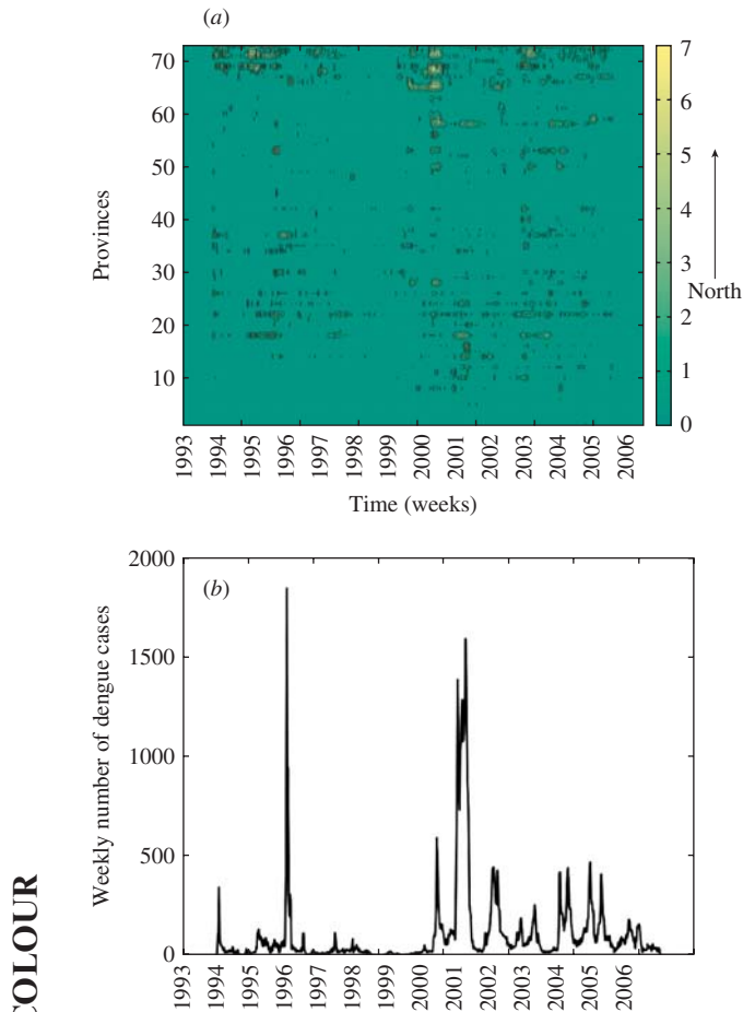
Fig. 2. (a) Weekly dengue incidence per 100 000 people in each of the 73 provinces [8] reporting dengue in Peru during the period 1994–2006. For visualization purposes, we took the log-transformation of the dengue incidence. Data were sorted by latitude coordinate from south to north. (b) The aggregated dengue epidemic curve of the new number of dengue cases by symptom onset during the period 1994–2006.
