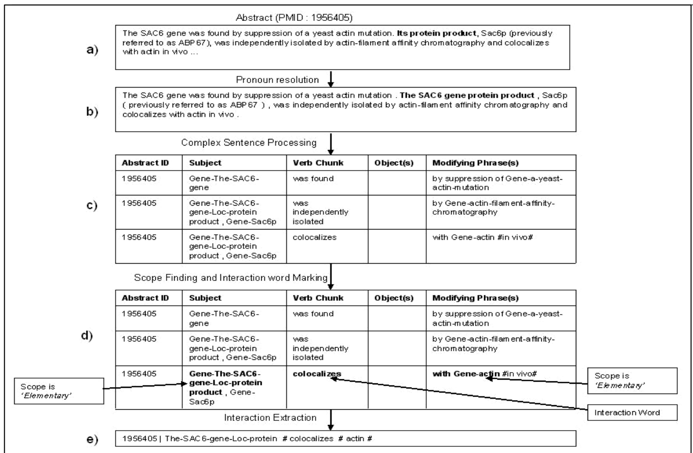
Fig. 3 Example - a) A Sentence from an abstract (PMID: 1956405). b) Pronoun 'it's' is resolved with 'The SAC6 gene'. c) Each row represents a simple sentence, d) for each constituent, role type is resolved and interaction words are tagged, e) Protein-Protein interaction is extracted.
