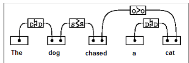
Figure 2: Link grammar representation of a sentence
