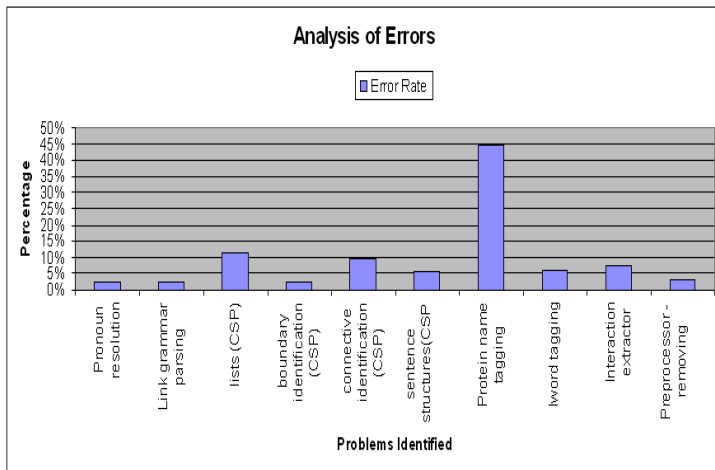
Figure 6: Analysis of types of errors encountered
