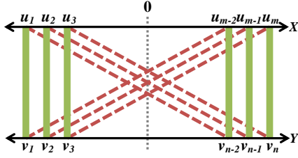
Fig. 1. Perfectly polarized bipartite graph
