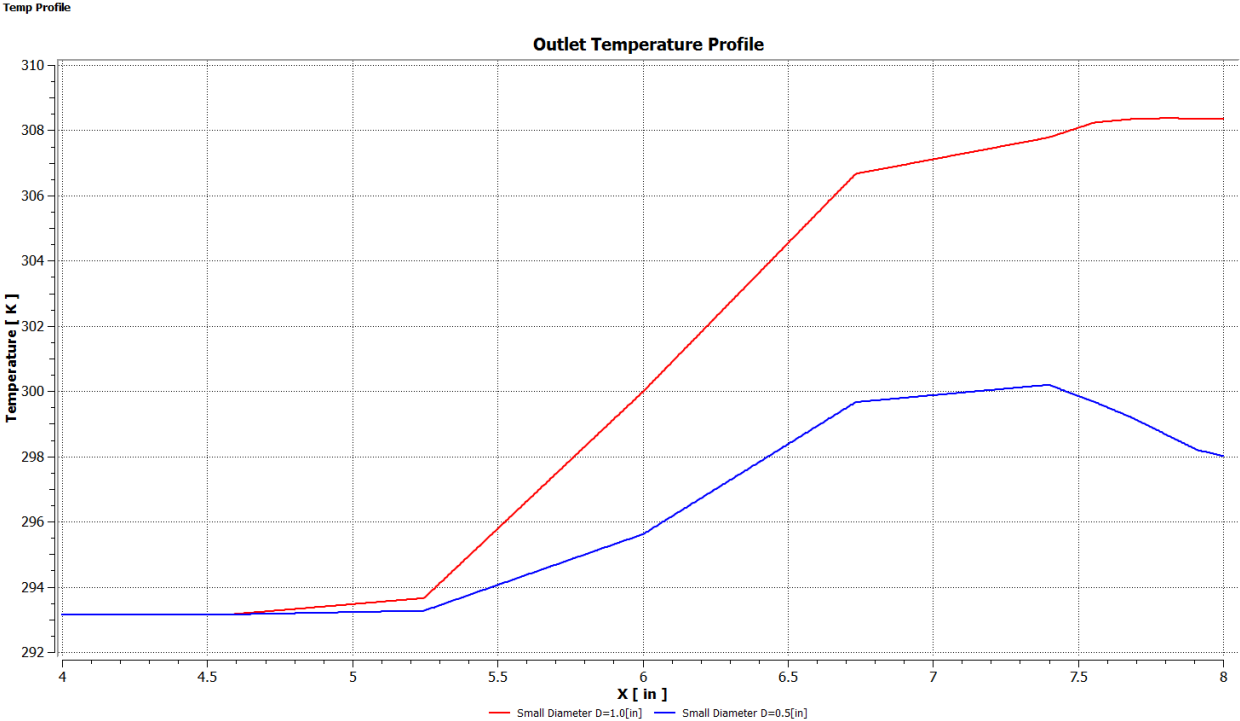
Figure 4: ANSYS CFD-Post displaying line AB temperature contours for both geometries. (Blue: Small inlet diameter of 0.5 [in], Red: Small inlet diameter of 1.0 [in])
