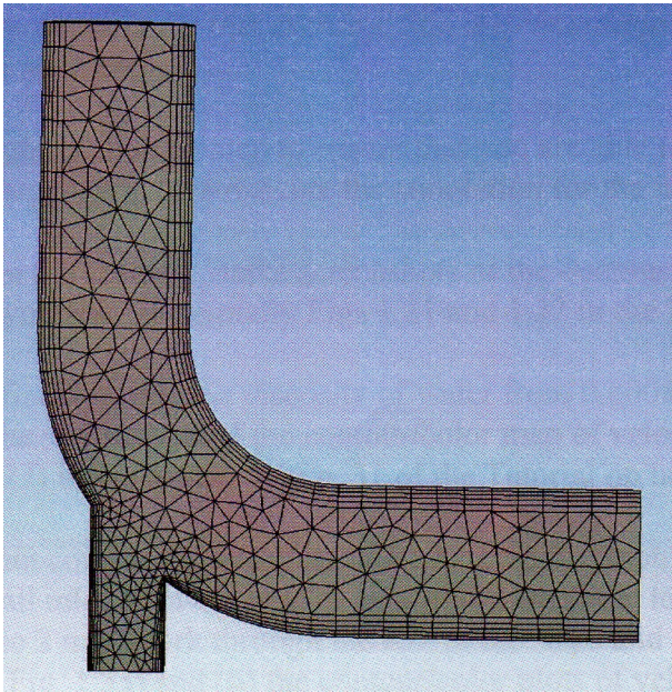
Screenshot of the mesh with an enlarged small inlet
