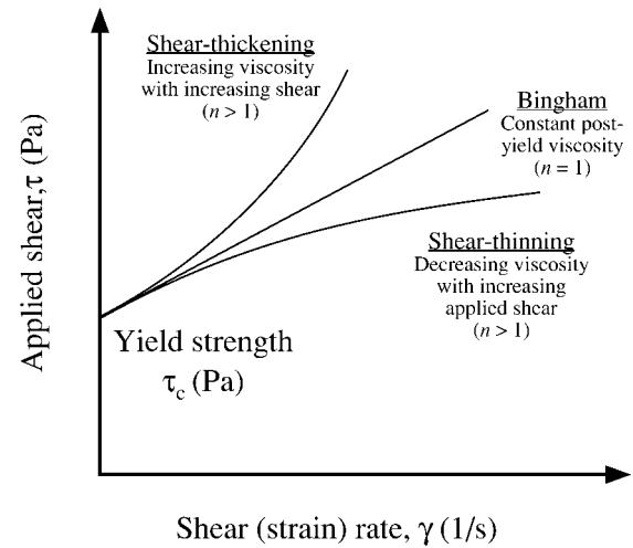
Figure 6. Diagram illustrating Bingham, shear-thinning, and shear-thickening behavior.
