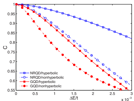
Fig. 2: (Color online) Autocorrelation C vs. energy difference \Delta E for different quantum dots with N_{\text{mode}}=48 .
