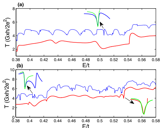
Fig. 1: (Color online) Transmission T vs. energy E for open (a) non-relativistic and (b) graphene quantum dot with the same maximum number of propagating modes: N_{\text{mode}}=24 . Blue/thin (red/thick) lines are for nonhyperbolic (hyperbolic) scattering dynamics in the classical limit. Note that, to clearly distinguish these two lines in each figure, we shift the transmissions for hyperbolic ones (red/thick) down by 1. The insets show the fitting lines (green) using eq. (1). The energy values E_0/t corresponding to the three cases are (a) 0.50581, (b/left) 0.40402, and (b/right) 0.53392.
