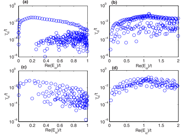
Fig. 3: (Color online) The real and imaginary part of the eigenstates E_\alpha for (a) GQD/nonhyperbolic, (b) NRQD/nonhyperbolic, (c) GQD/hyperbolic, and (d) NRQD/hyperbolic. The energy values E_0 in (a)–(d) are 0.2, 1, 0.2 and 1, respectively.
