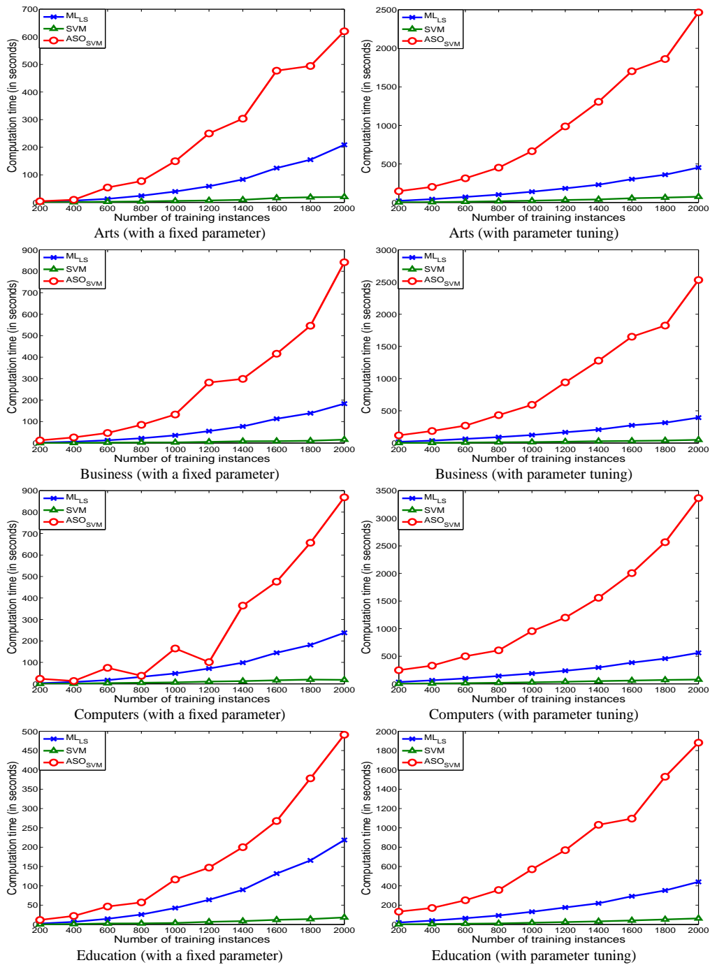
Fig. 1. Comparison of computation time for ML LS , SVM, and ASO SVM on four Yahoo! data sets. The computation time for a fixed parameter setting and that for parameter tuning using cross-validation are both depicted for each data set. See the text for more details.
