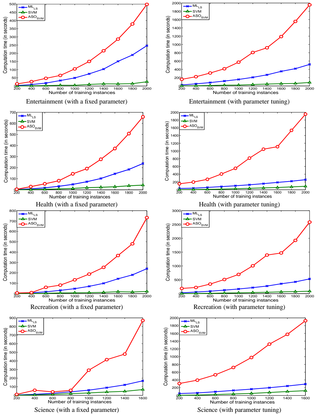
Fig. 2. Comparison of computation time for ML_{LS} , SVM, and ASO_{SVM} on four Yahoo! data sets. The computation time for a fixed parameter setting and that for parameter tuning using cross-validation are both depicted for each data set. See the text for more details.
