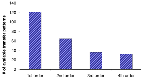
Figure 1: Number of recognizable group transfer patterns vs. Markov order for AIX problems
