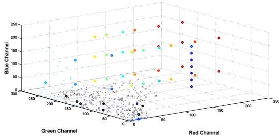
Figure 3. Visualization of quantization of AutoCC approach proposed in [7].
