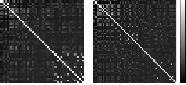
Figure 2: The Pearson’s correlation coefficients computed on the columns of the label indicator matrix using two data sets from stage range 11-12 (left figure) and 13-16 (right figure) with 50 and 60 terms, respectively.
