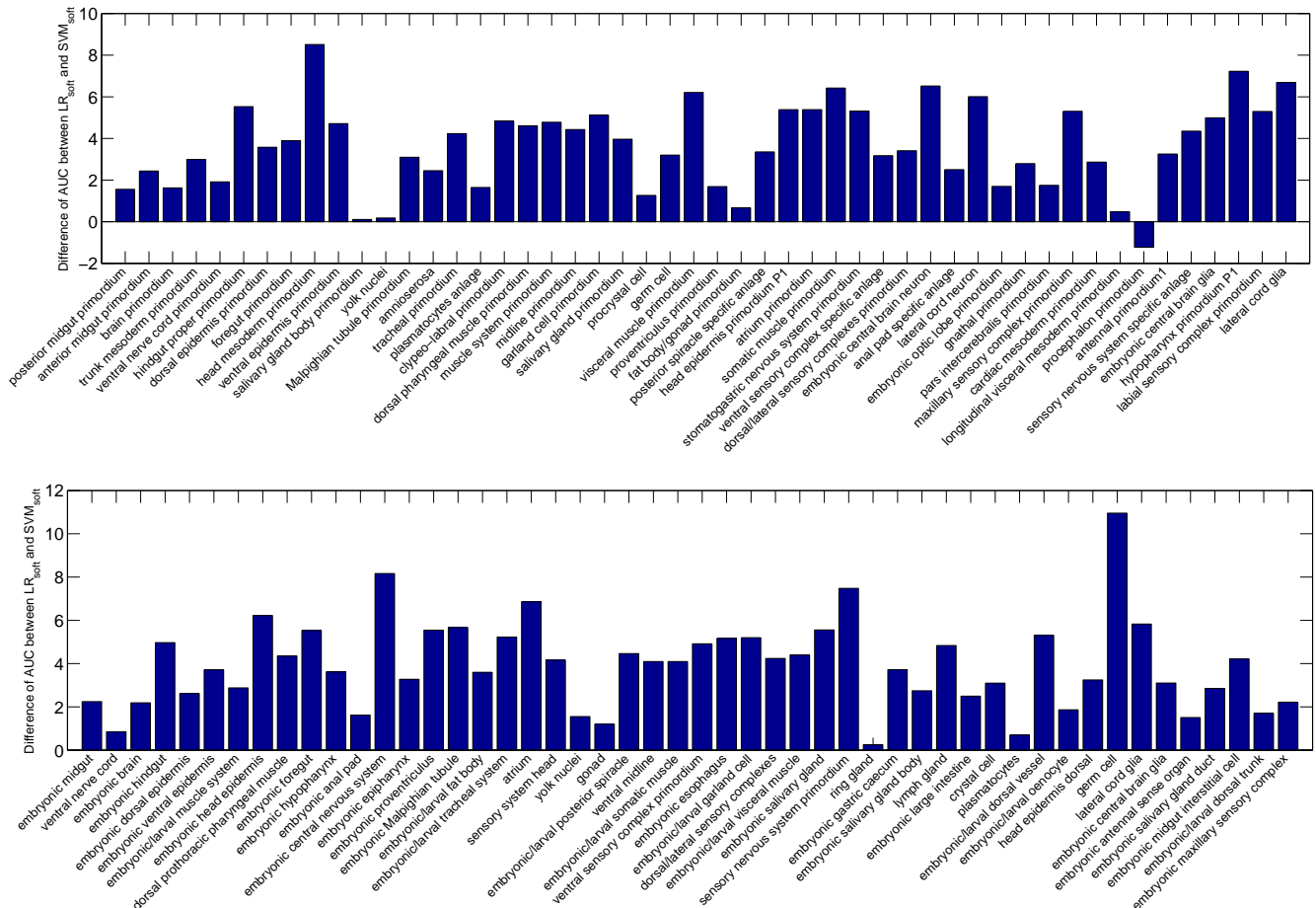
Figure 4: Performance differences on individual terms in terms of AUC between LR_{\text{soft}} and SVM_{\text{soft}} on two data sets from stage range 11-12 (top) and 13-16 (bottom) with 50 terms. Positive bar values show that LR_{\text{soft}} outperforms SVM_{\text{soft}} and negative bar values show that SVM_{\text{soft}} outperforms LR_{\text{soft}} .
