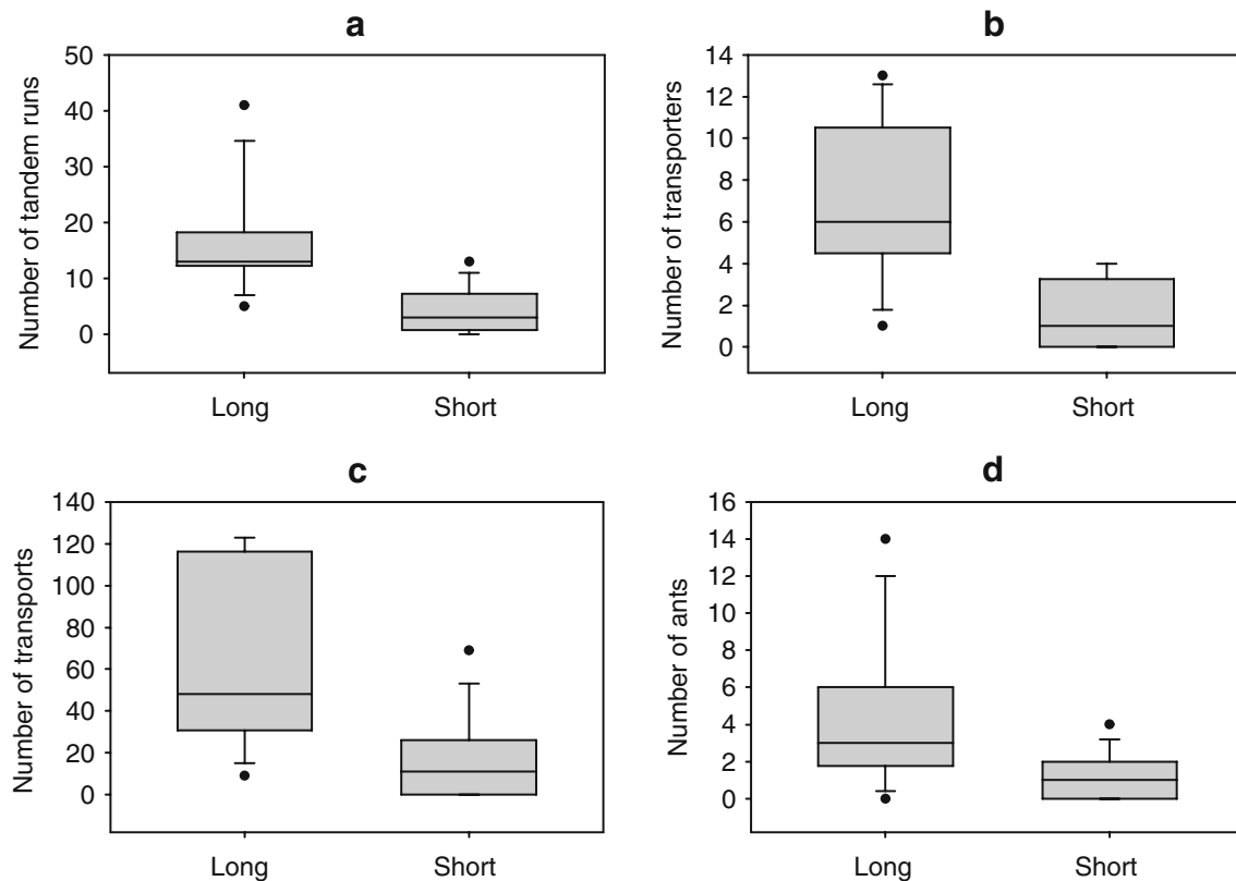
Fig. 3 Comparison of tandem run contribution to long and short emigrations. a The total number of tandem run followers was significantly greater in the long treatment (Wilcoxon test: W=75.5 , n=18 , p<0.01 ), as were b the number of transporters recruited in tandem runs (Wilcoxon test: W=73.0 , n=18 , p<0.01 ), c the number of transports completed by ants recruited in tandem runs (Wilcoxon test:
