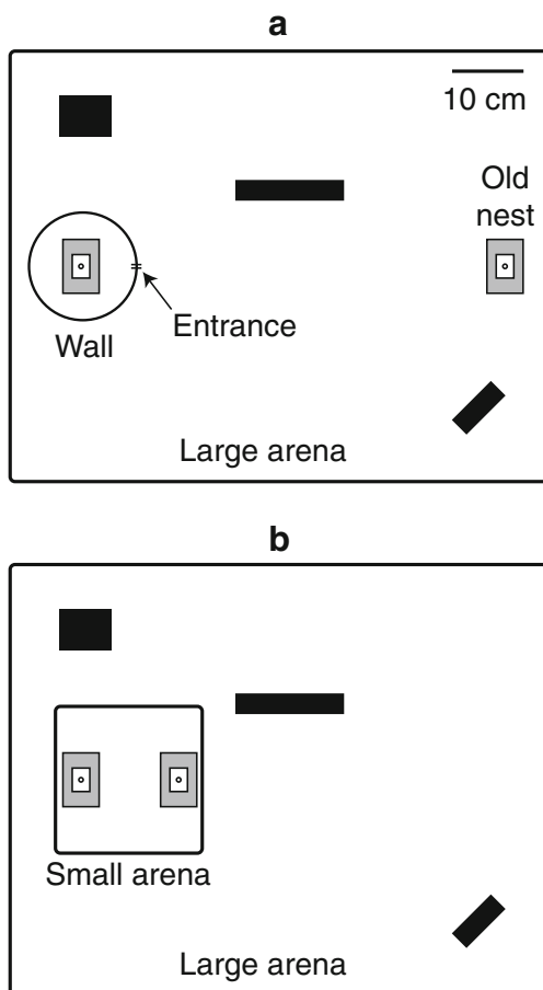
Fig. 1 Layout of emigration arenas. a In the long treatment, the new nest was hidden within a circular enclosure accessible by a single small entrance hole. Black rectangles show the locations of visual landmarks. b In the short treatment, ants moved in a smaller arena to an unconcealed nest. The small arena was placed inside the large one to give similar visual cues in each treatment
