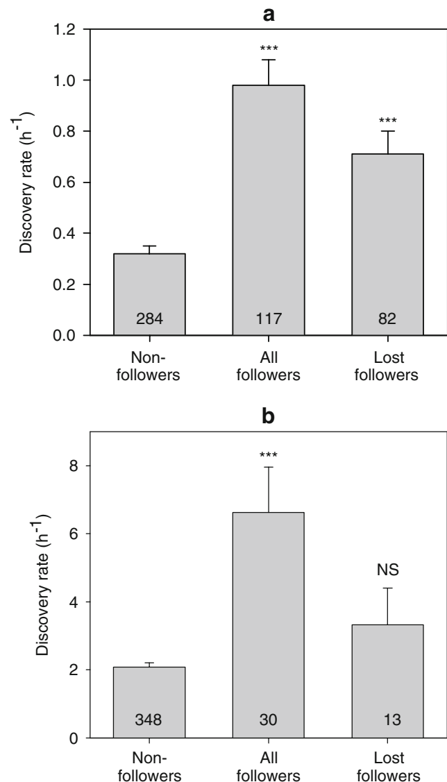
Fig. 2 Comparison of per capita nest discovery rates for ants that followed tandem runs and ants that did not. The discovery rate of followers was measured twice: once using all followers and once using only those that lost contact with their tandem leader. a In the long treatment, the rate for nonfollowers was significantly exceeded by the rates for all followers ( \chi_1^2 = 74.4 , n=401 , p<0.0001 ) and for lost followers ( \chi_1^2 = 29.9 , n=366 , p<0.0001 ). b In the short treatment, the rate for nonfollowers was significantly exceeded by the rate for all followers ( \chi_1^2 = 27.0 , n=378 , p<0.0001 ) but not by the rate for lost followers ( \chi_1^2 = 2.4 , n=361 , p=0.12 ). Numbers on bars give sample sizes
