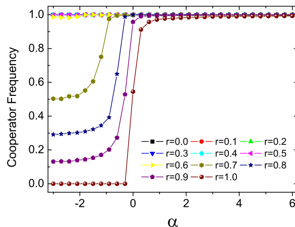
Fig. 2: (Color online) Frequency of cooperators as a function of the asymmetric parameter \alpha for different values of the total cost r on scale-free networks.
