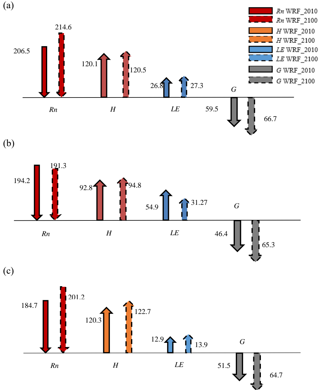
Figure 3.13. Impact of urban expansion on the energy balance of urban surface over daytime for (a) Phoenix, (b) Denver, and (c) Las Vegas. R_n is the net radiation (positive downwards); H is sensible heat (positive upwards); LE is latent heat (positive upwards); G is the ground heat (negative downwards). All values are in W/m^2 .
