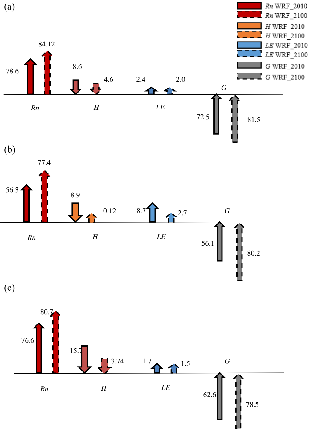
Figure 3.14. Impact of urban expansion on the energy balance of urban surface over nighttime for (a) Phoenix, (b) Denver, and (c) Las Vegas. R_n is the net radiation (positive downwards); H is sensible heat (positive upwards); LE is latent heat (positive upwards); G is the ground heat (negative downwards). All values are in W/m^2 .
