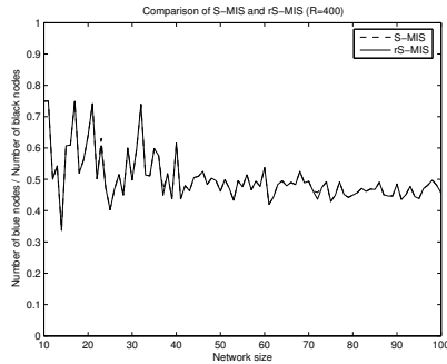
(a) Performance comparison of S-MIS and rS-MIS
