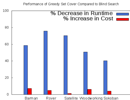
Figure 5: The graph compares the performance of greedy set cover against the optimal blind search for |F| = 4 . It plots the average time saved by the set cover and the average increase in cost of the solution for each domain.
